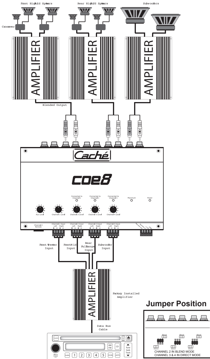
coe8 configuration for an active 2 way front, plus rear input system using the blend mode on channel 2.
