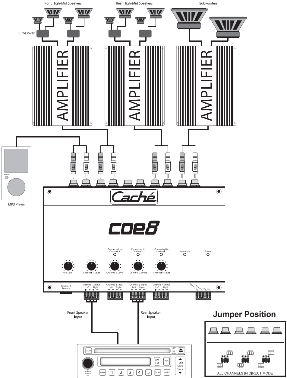
coe8 configuration for a full range high level 4 channel input system in direct mode.
