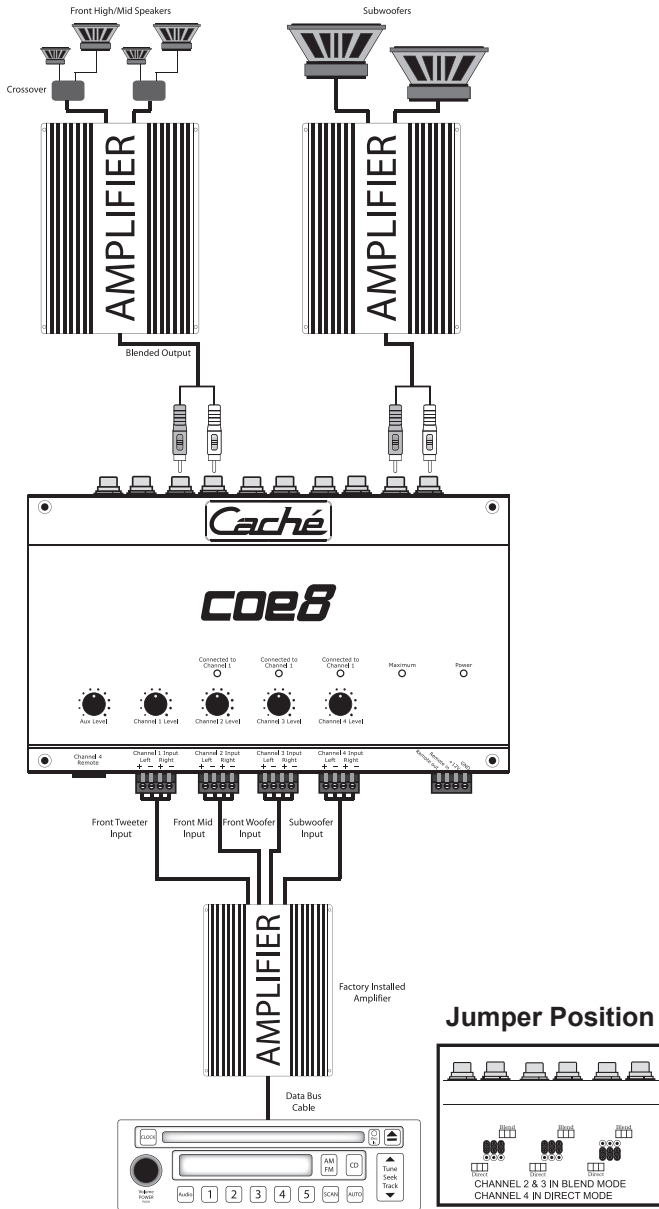
coe8 configuration for an active 3 way front, plus sub input system using the blend mode on channels 2 & 3.
